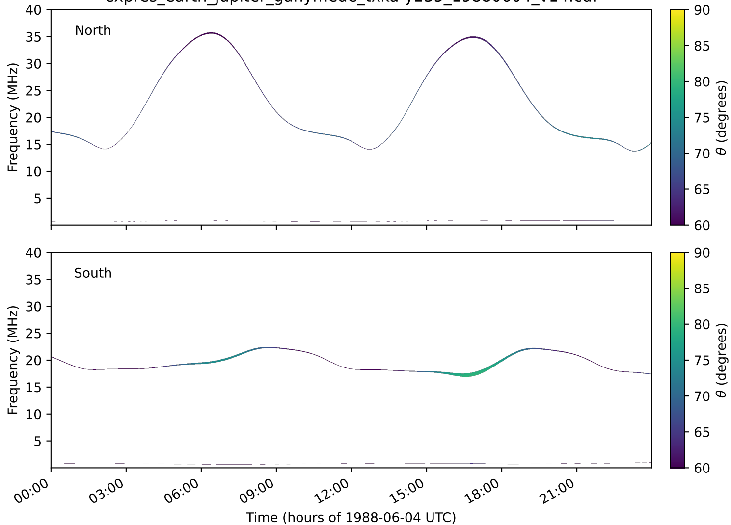
expres_earth_jupiter_ganymede_txka-y235_19880604_v14.cdf
