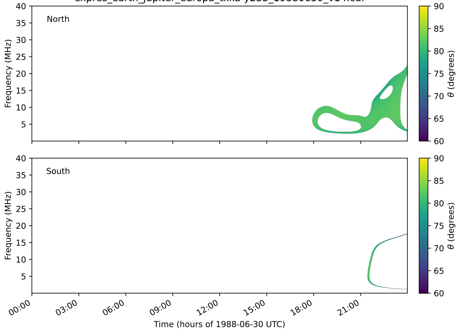
expres_earth_jupiter_europa_txka-y235_19880630_v14.cdf
