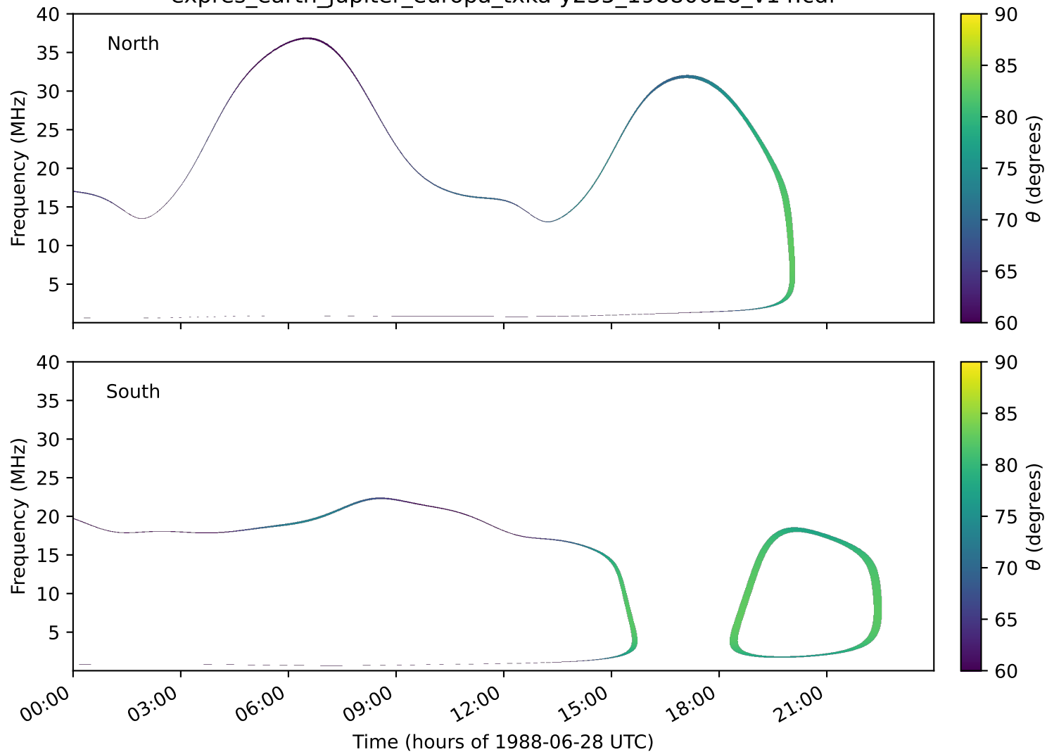
expres_earth_jupiter_europa_txka-y235_19880628_v14.cdf
