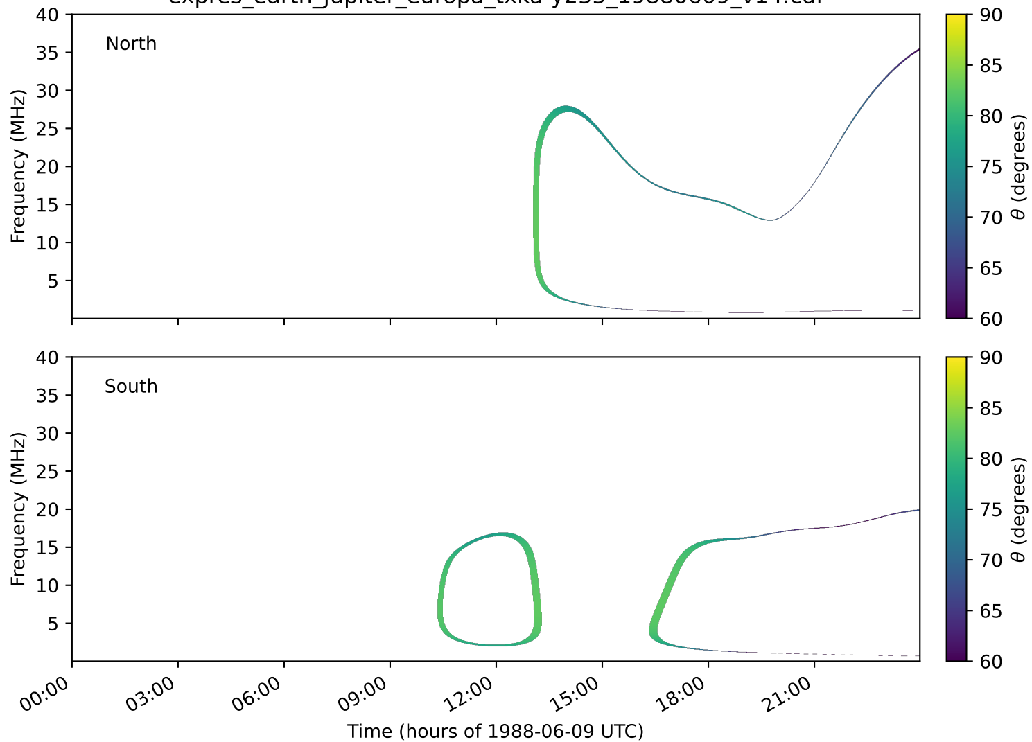
expres_earth_jupiter_europa_txka-y235_19880609_v14.cdf
