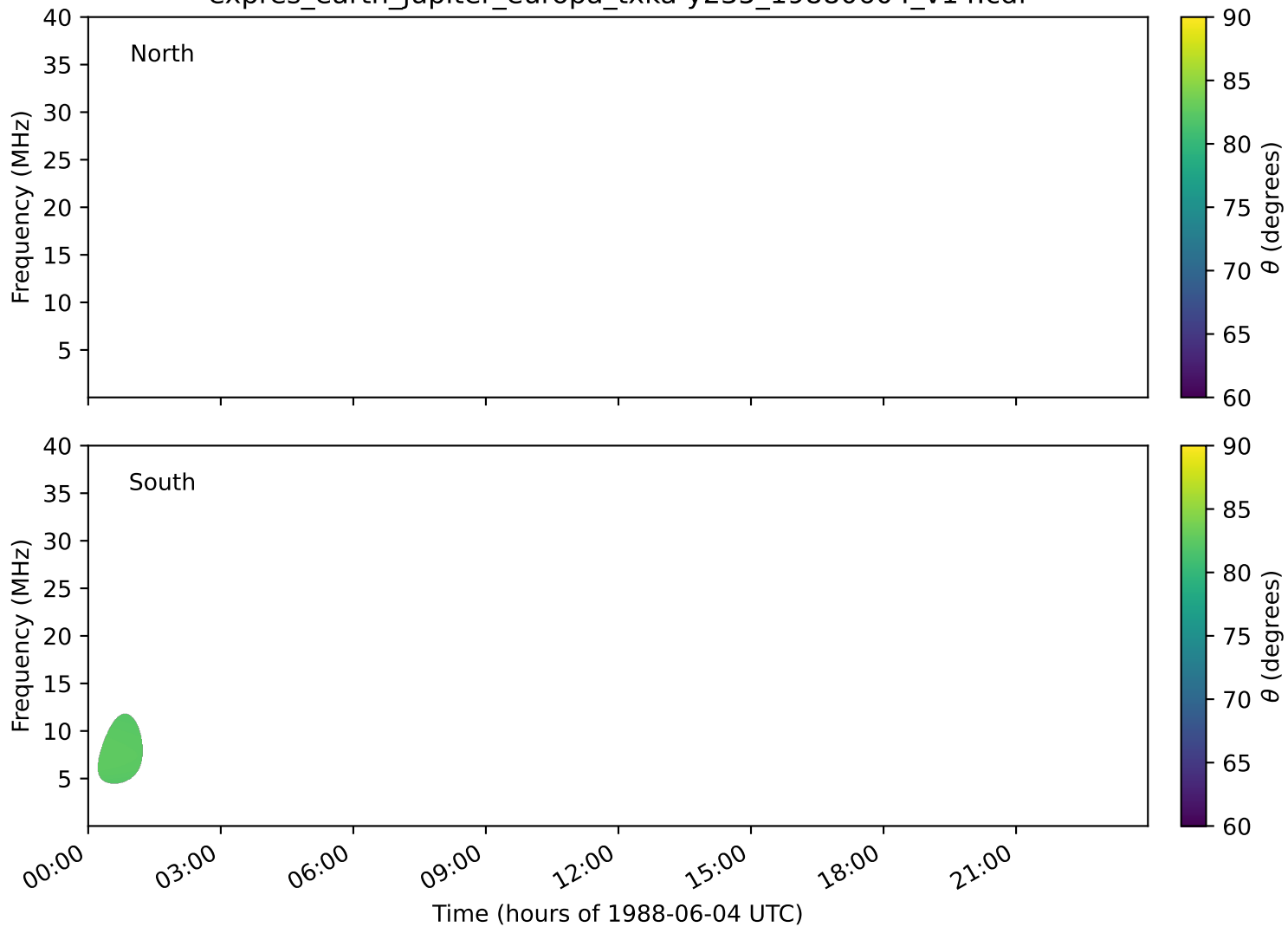
expres_earth_jupiter_europa_txka-y235_19880604_v14.cdf
