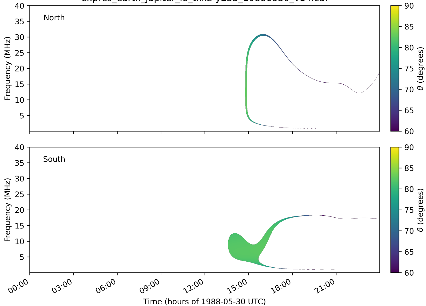
expres_earth_jupiter_io_txka-y235_19880530_v14.cdf
