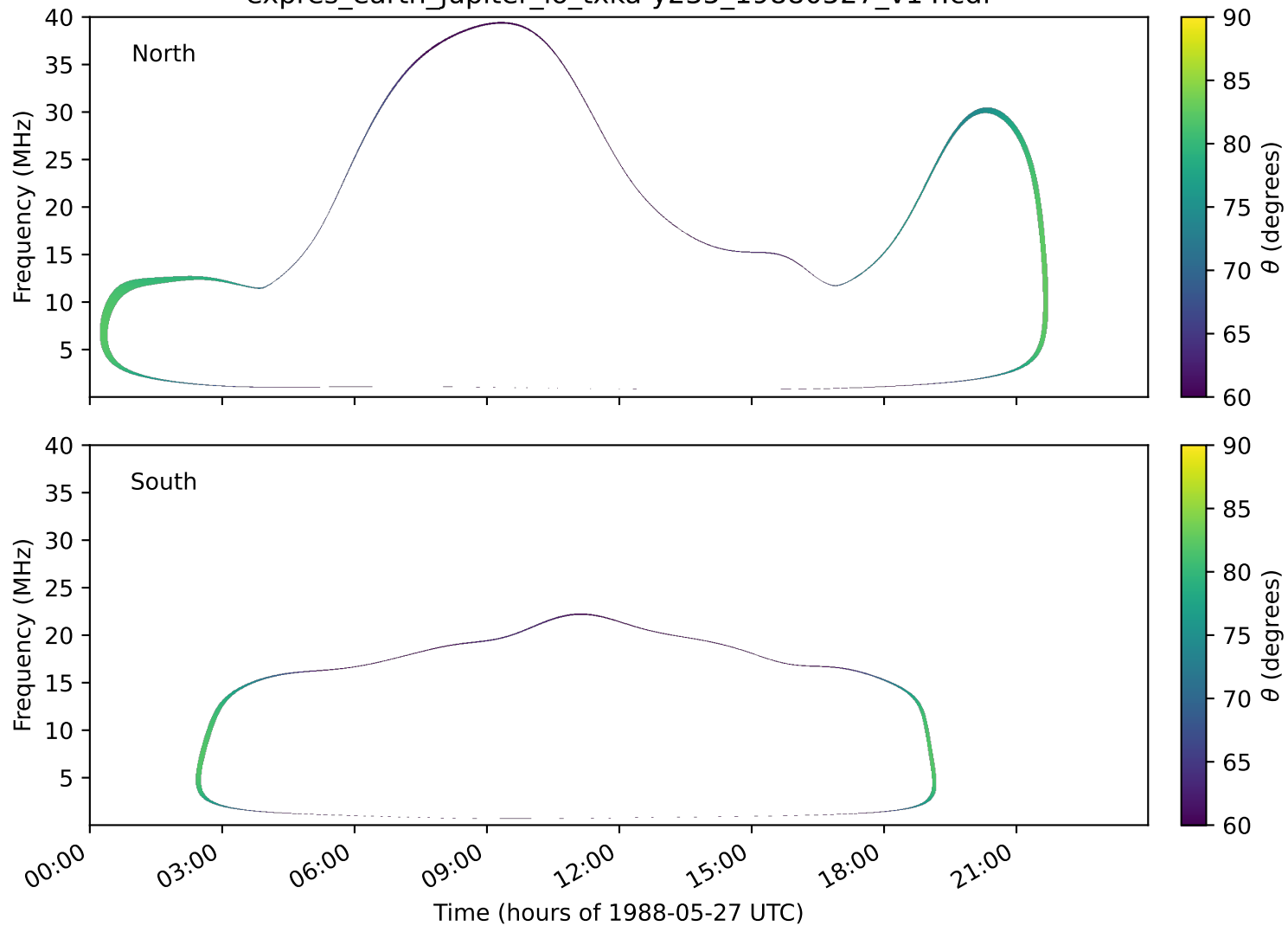
expres_earth_jupiter_io_txka-y235_19880527_v14.cdf
