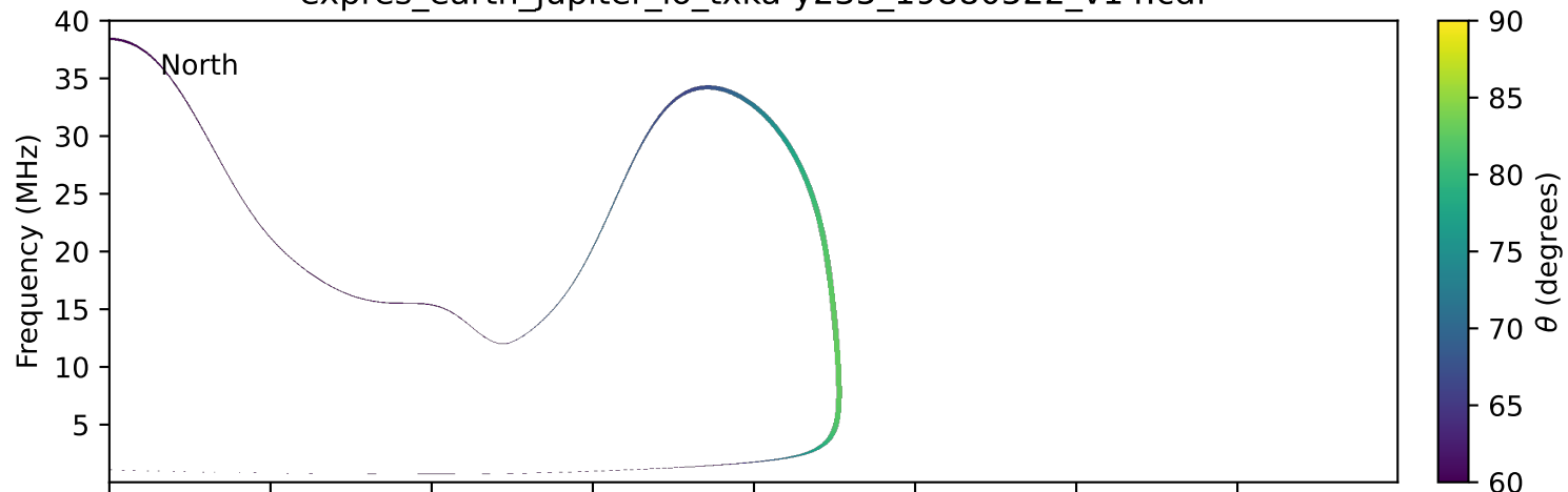
expres_earth_jupiter_io_txka-y235_19880522_v14.cdf
