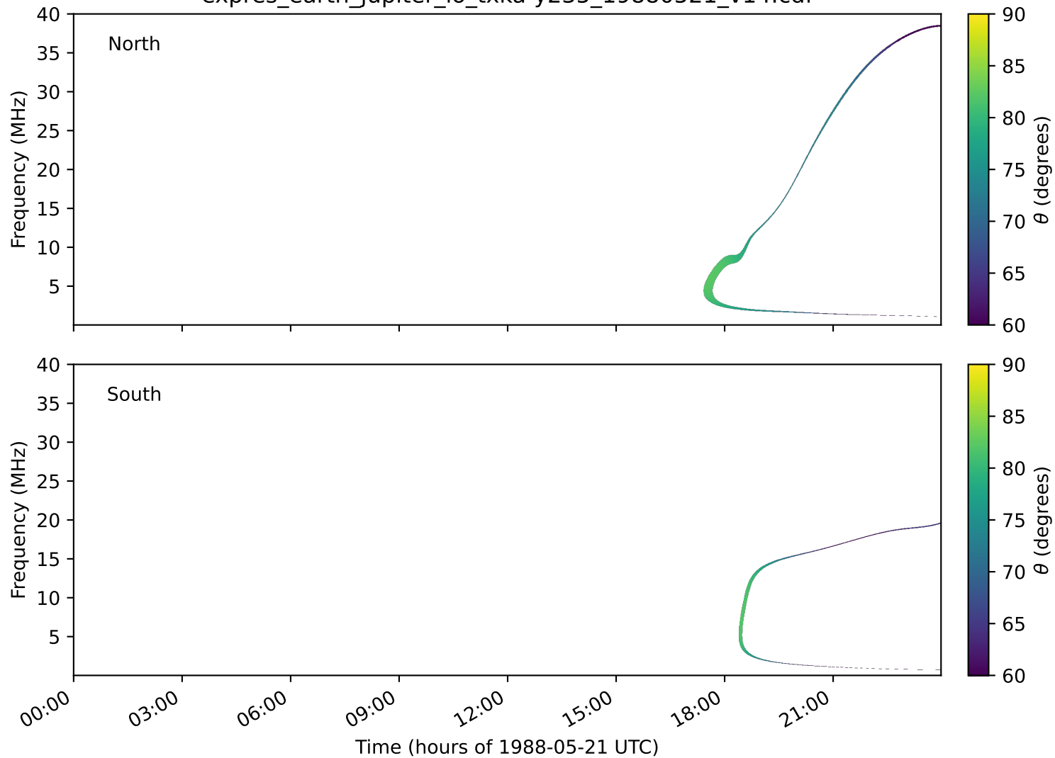
expres_earth_jupiter_io_txka-y235_19880521_v14.cdf
