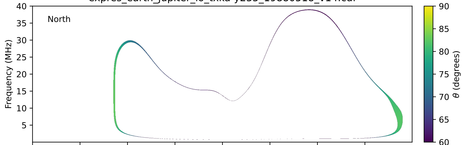
expres_earth_jupiter_io_txka-y235_19880518_v14.cdf
