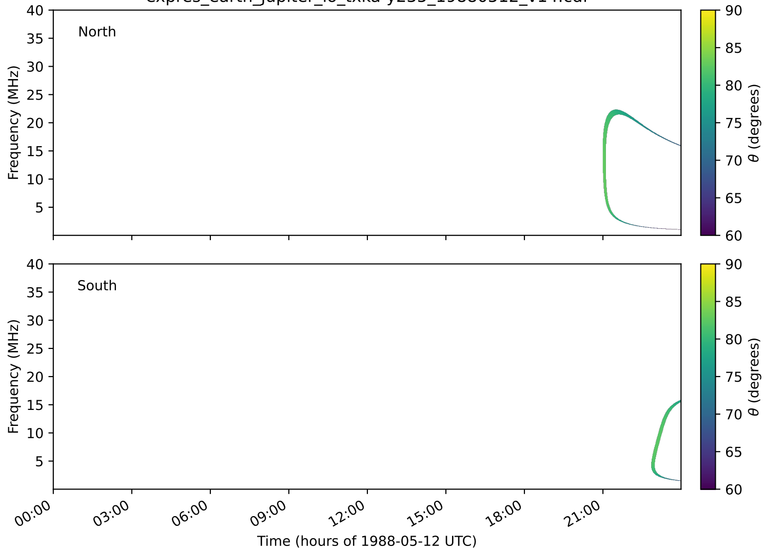
expres_earth_jupiter_io_txka-y235_19880512_v14.cdf
