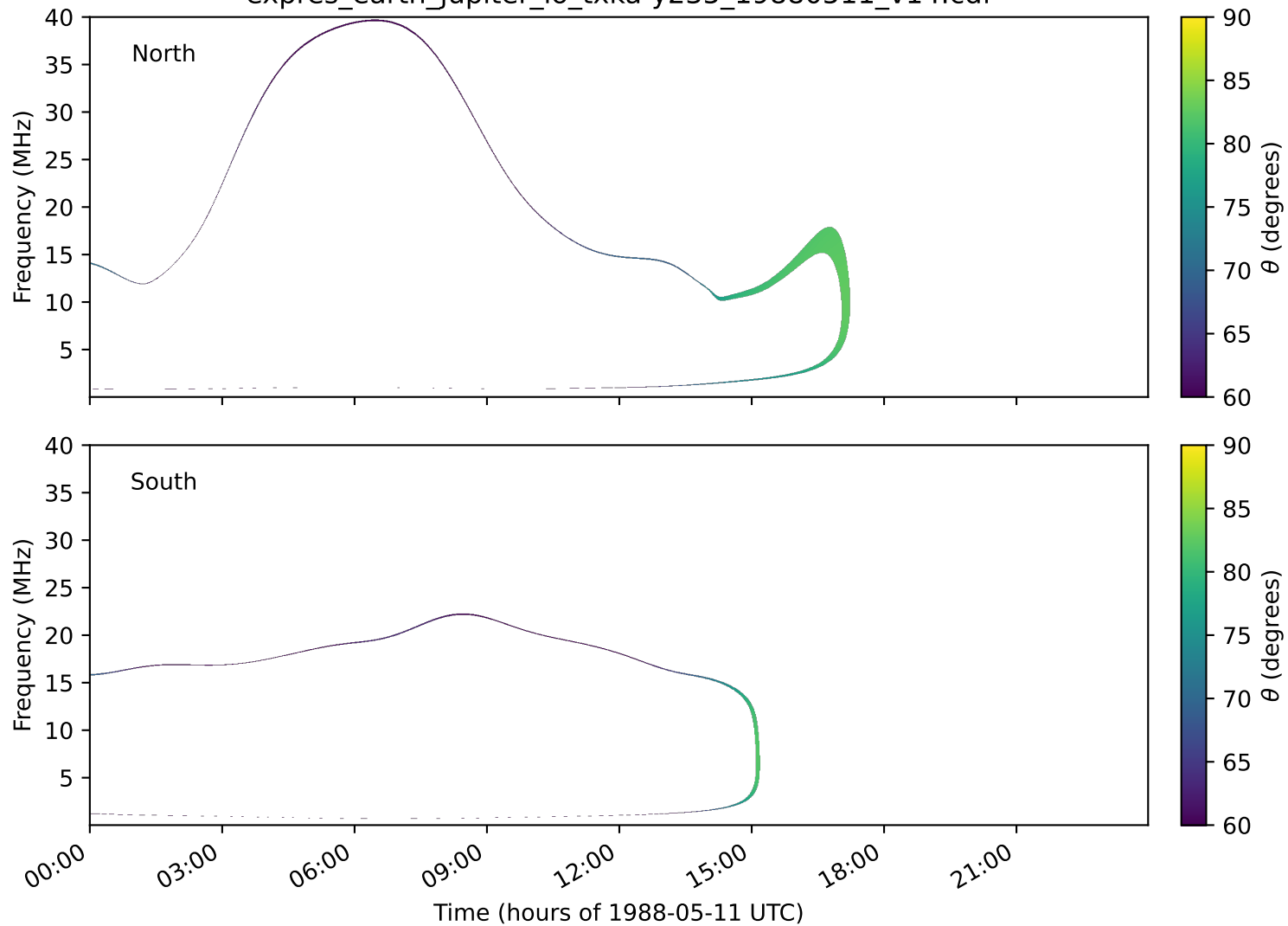
expres_earth_jupiter_io_txka-y235_19880511_v14.cdf
