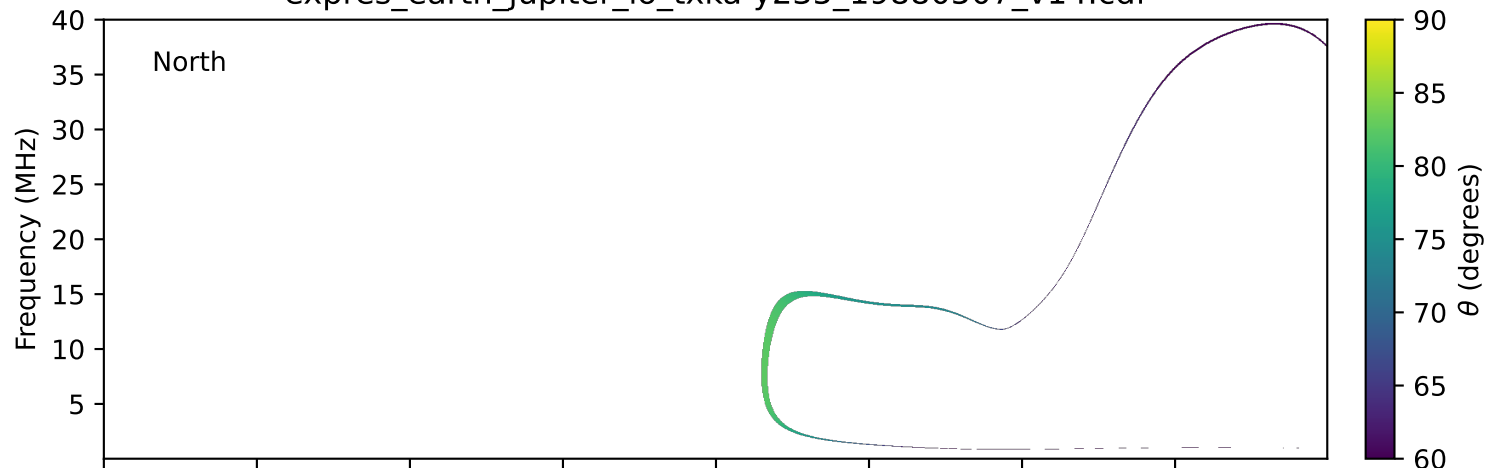
expres_earth_jupiter_io_txka-y235_19880507_v14.cdf
