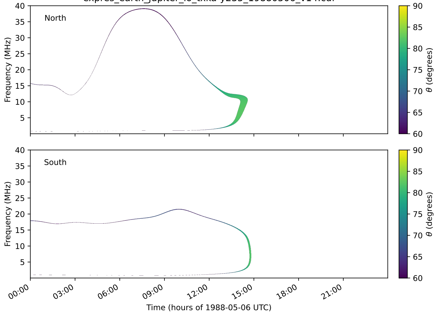
expres_earth_jupiter_io_txka-y235_19880506_v14.cdf
