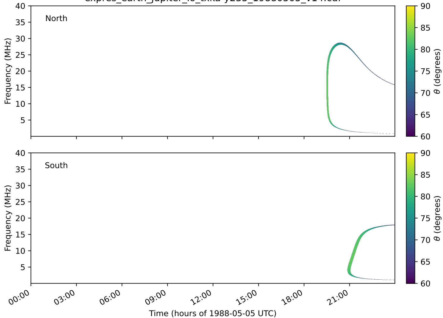
expres_earth_jupiter_io_txka-y235_19880505_v14.cdf
