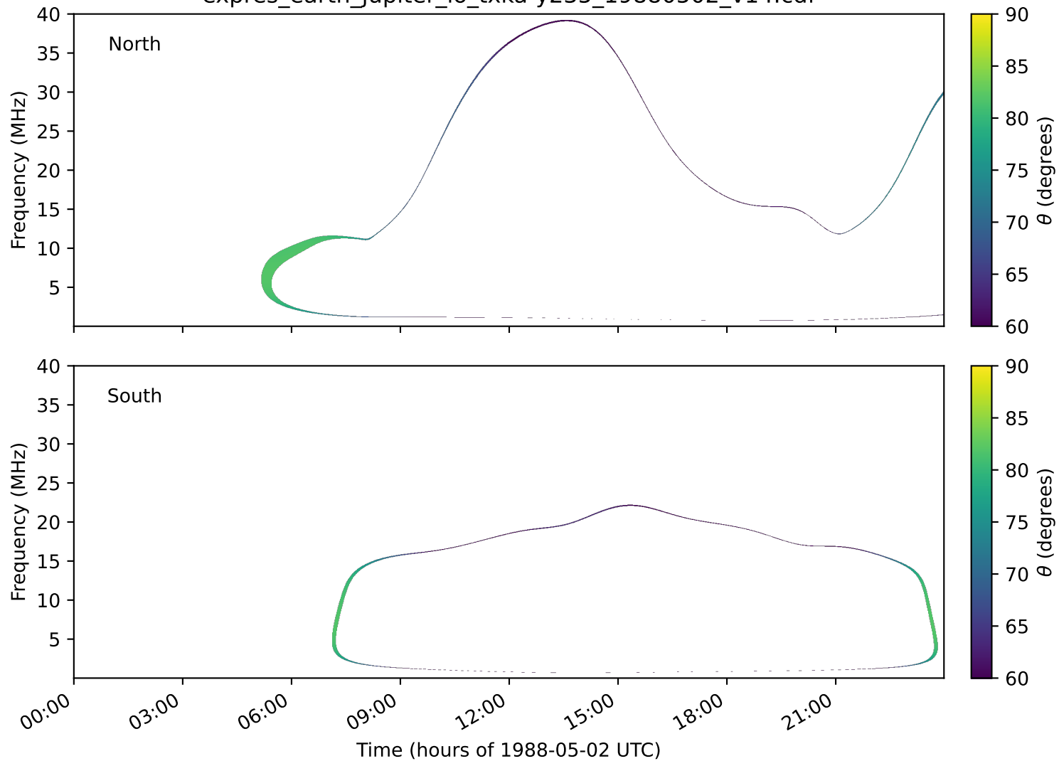
expres_earth_jupiter_io_txka-y235_19880502_v14.cdf
