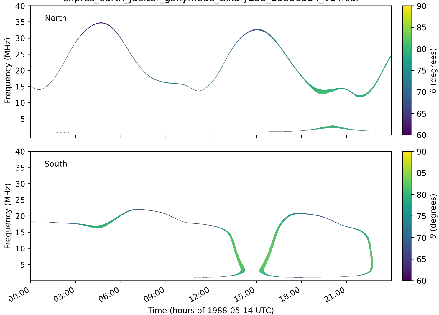
expres_earth_jupiter_ganymede_txka-y235_19880514_v14.cdf
