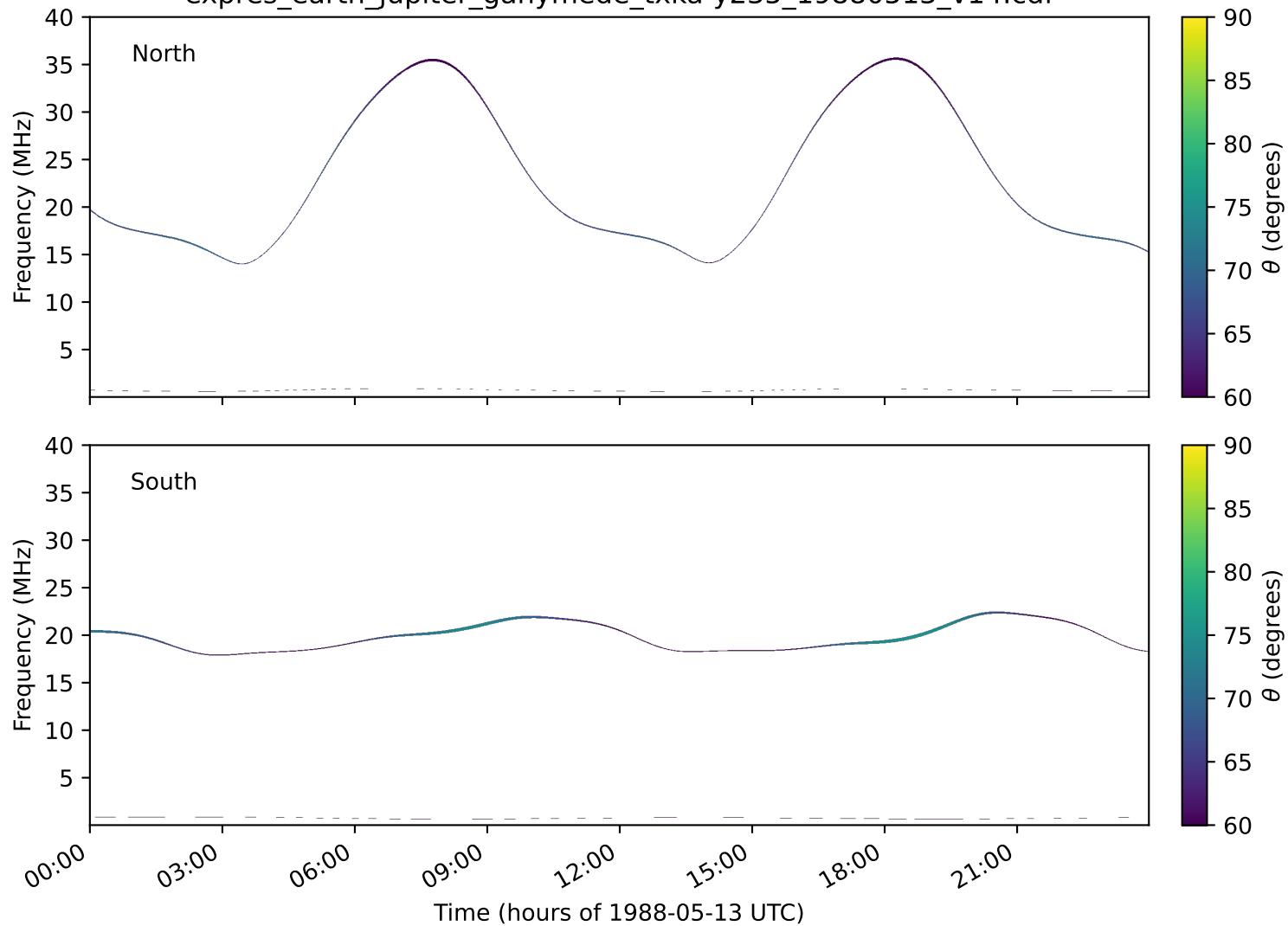
expres_earth_jupiter_ganymede_txka-y235_19880513_v14.cdf
