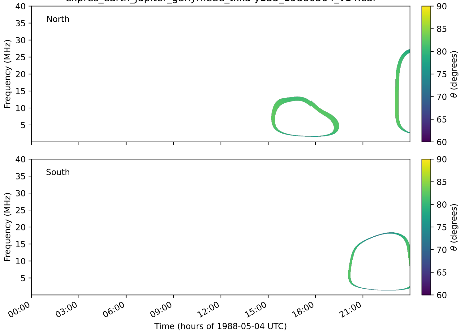
expres_earth_jupiter_ganymede_txka-y235_19880504_v14.cdf
