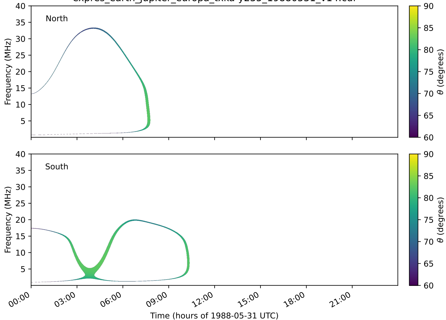
expres_earth_jupiter_europa_txka-y235_19880531_v14.cdf
