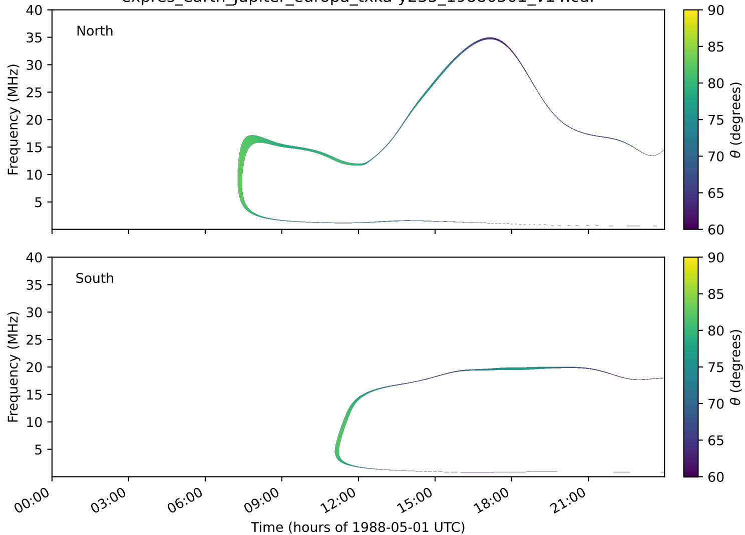
expres_earth_jupiter_europa_txka-y235_19880501_v14.cdf
