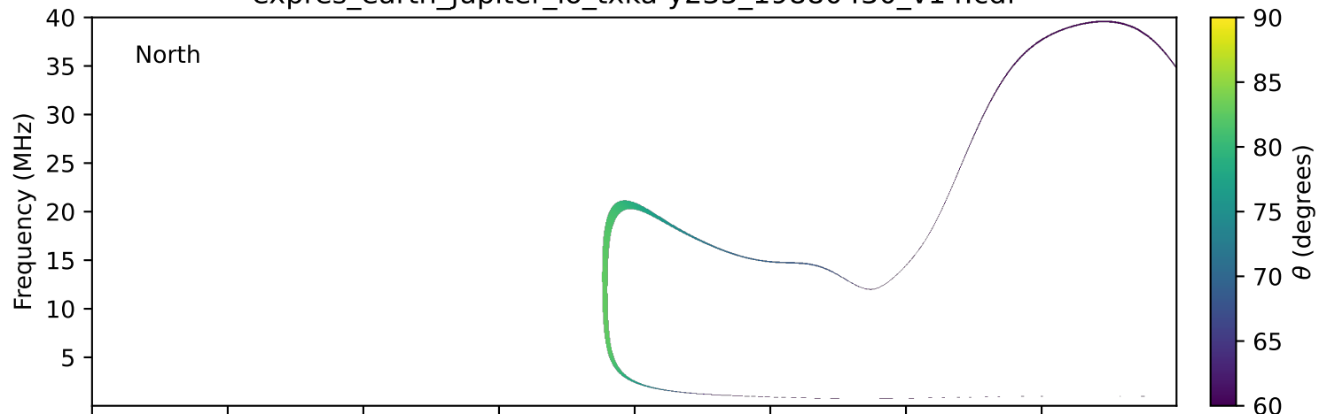
expres_earth_jupiter_io_txka-y235_19880430_v14.cdf
