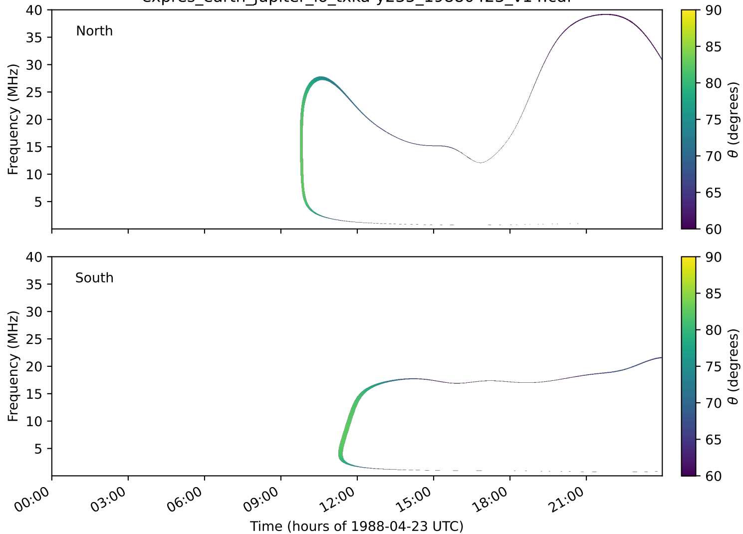
expres_earth_jupiter_io_txka-y235_19880423_v14.cdf
