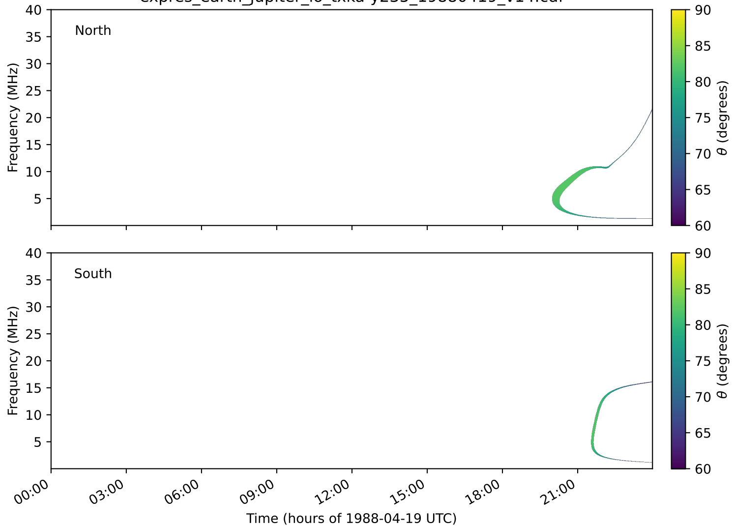
expres_earth_jupiter_io_txka-y235_19880419_v14.cdf
