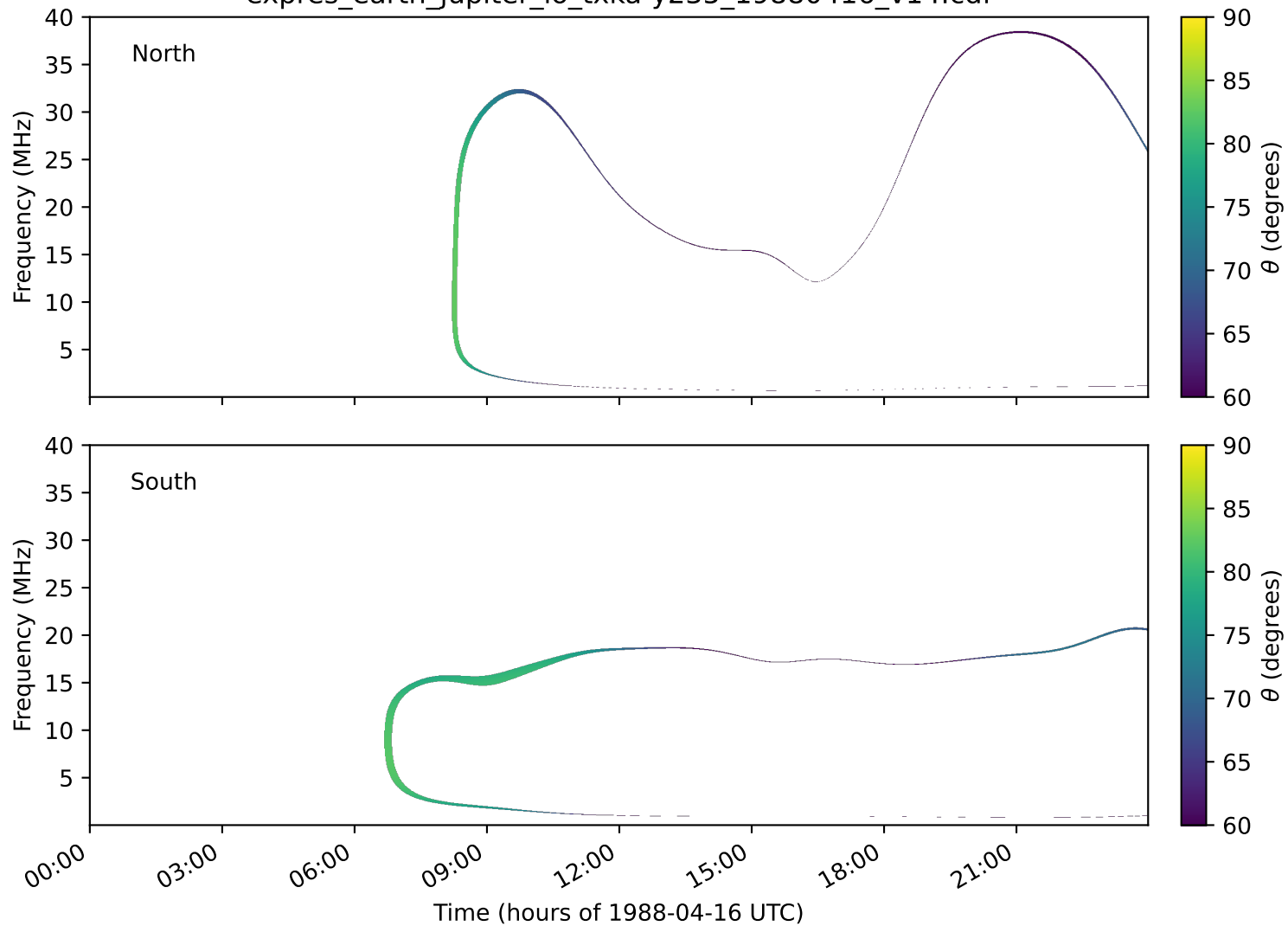
expres_earth_jupiter_io_txka-y235_19880416_v14.cdf
