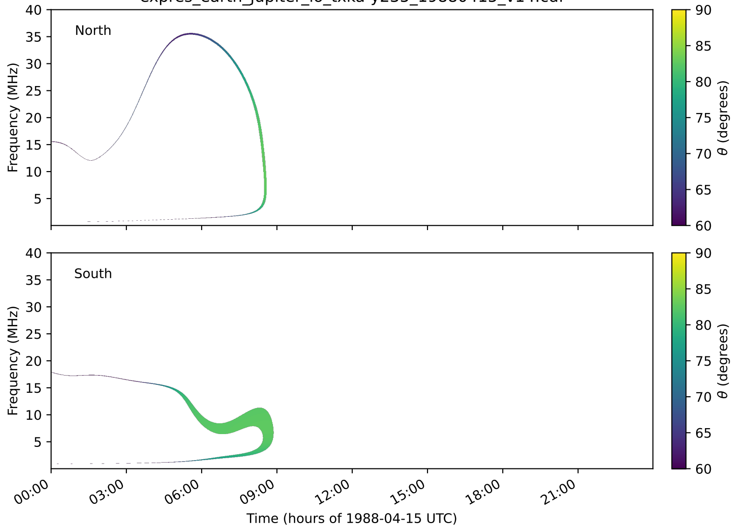
expres_earth_jupiter_io_txka-y235_19880415_v14.cdf
