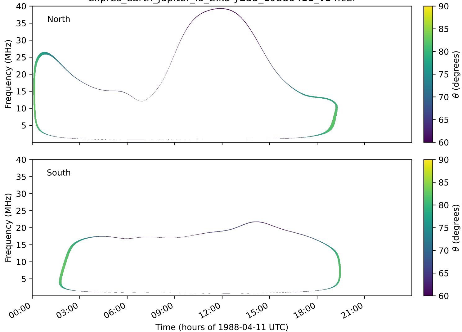
expres_earth_jupiter_io_txka-y235_19880411_v14.cdf
