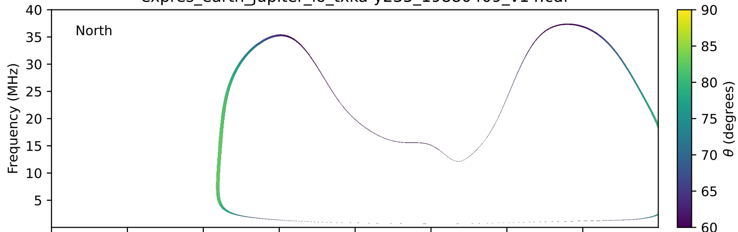
expres_earth_jupiter_io_txka-y235_19880409_v14.cdf
