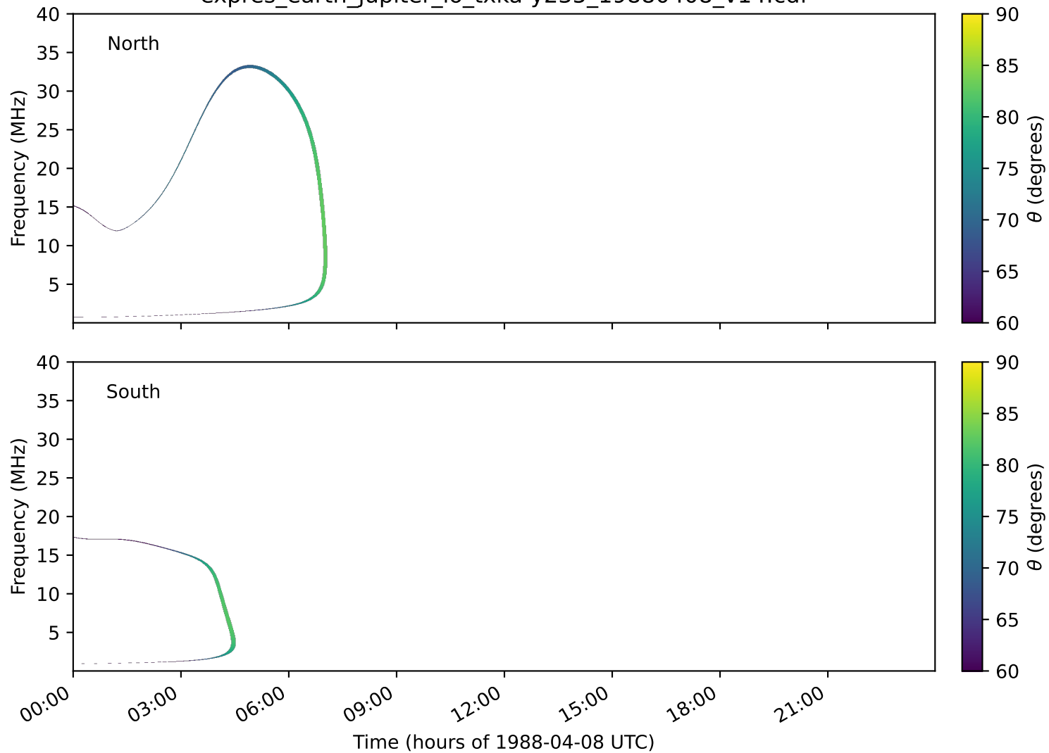
expres_earth_jupiter_io_txka-y235_19880408_v14.cdf
