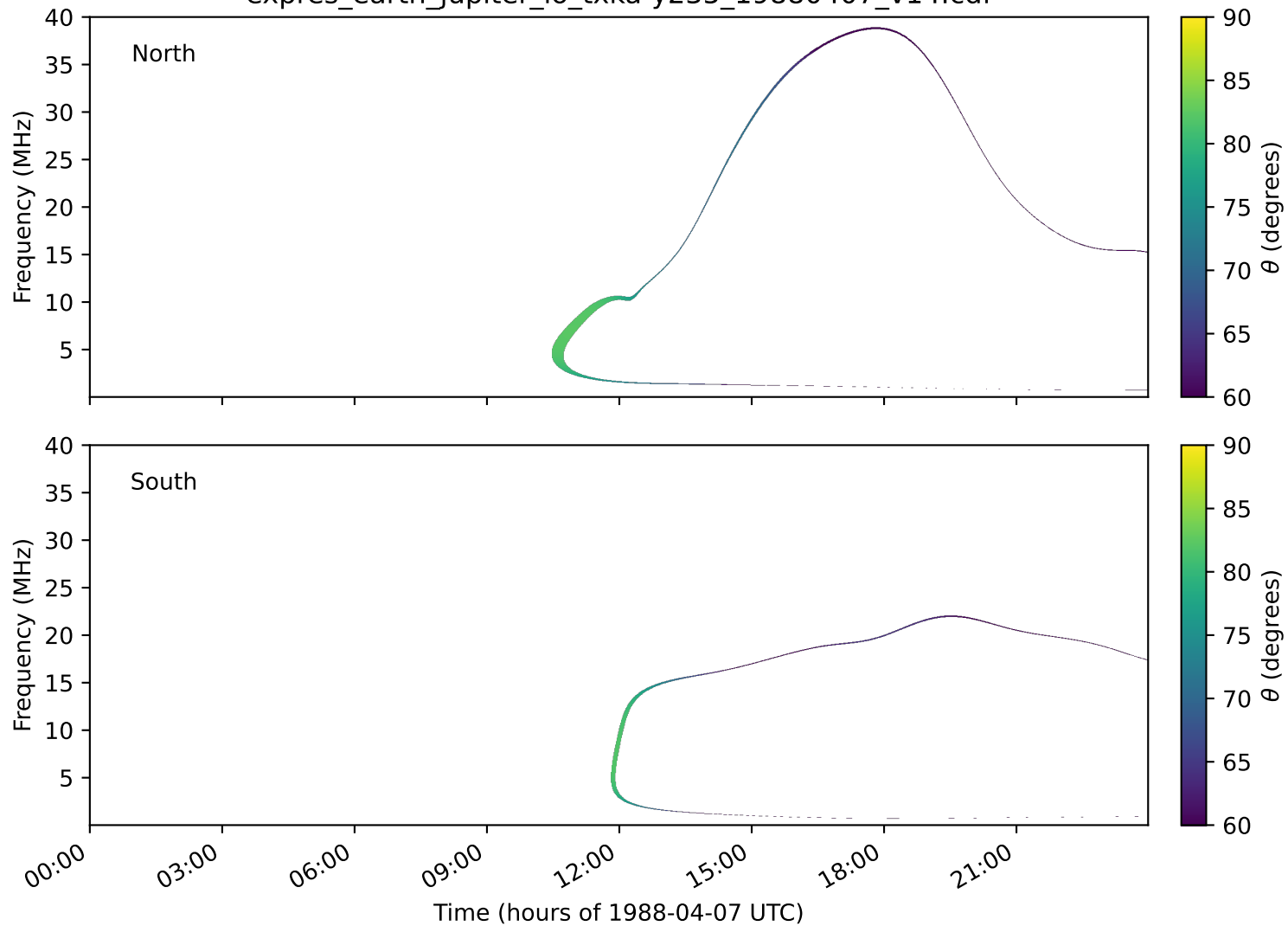
expres_earth_jupiter_io_txka-y235_19880407_v14.cdf
