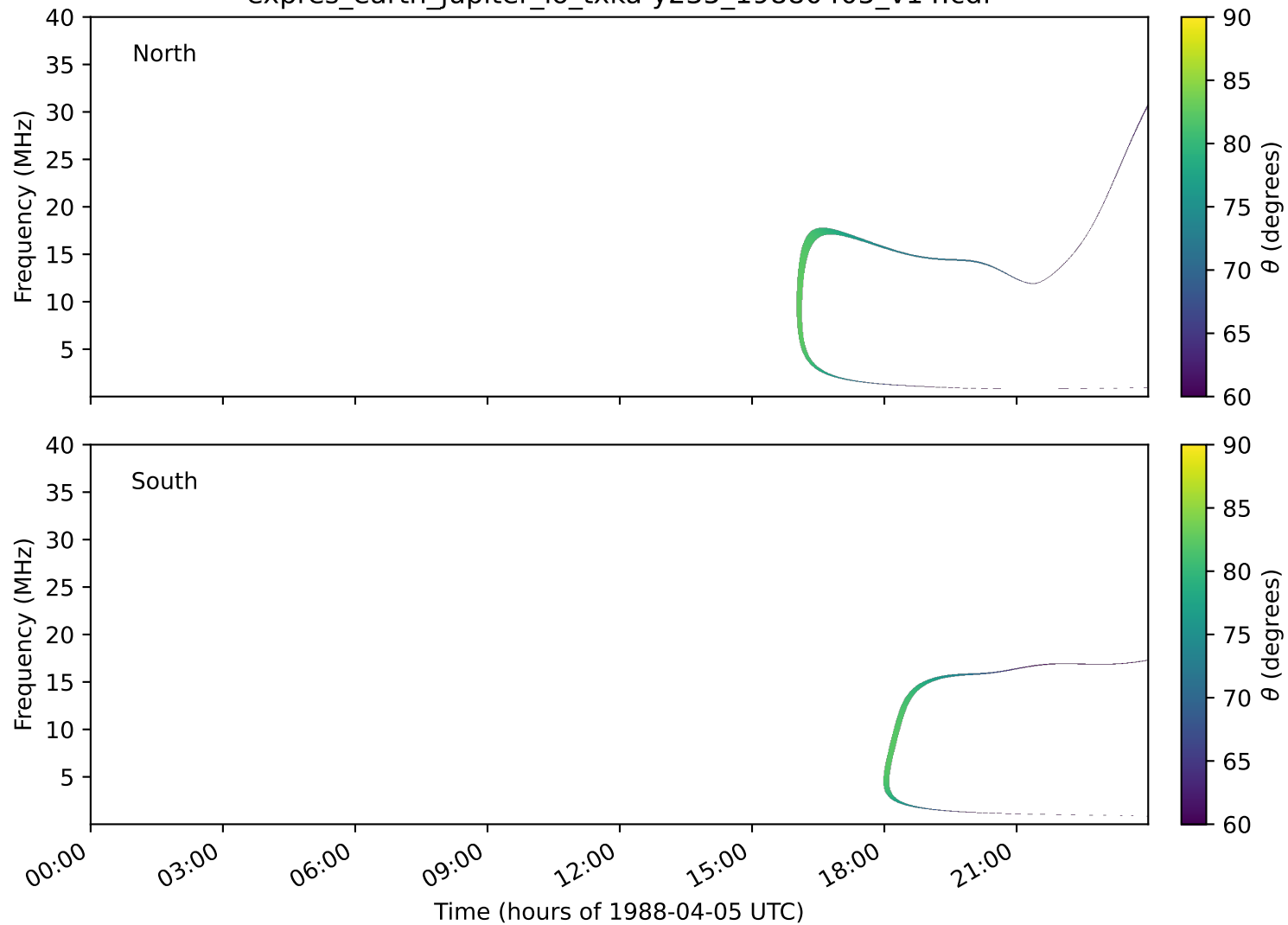
expres_earth_jupiter_io_txka-y235_19880405_v14.cdf
