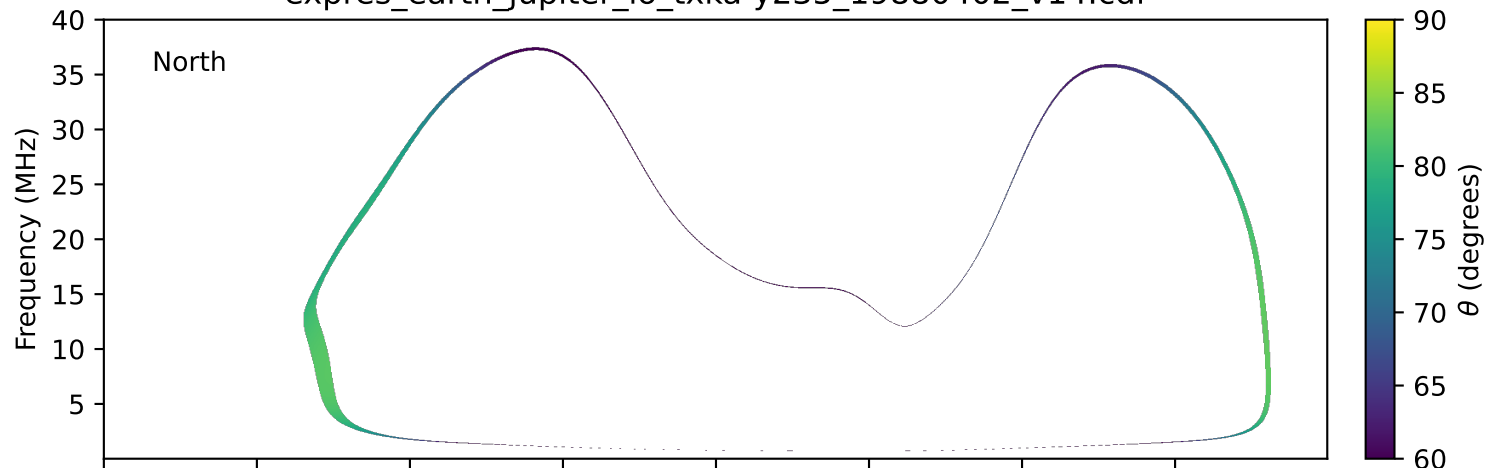
expres_earth_jupiter_io_txka-y235_19880402_v14.cdf
