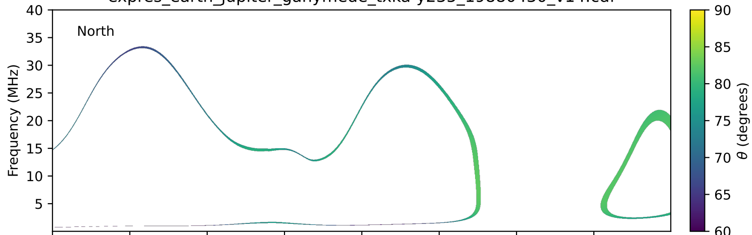
expres_earth_jupiter_ganymede_txka-y235_19880430_v14.cdf
