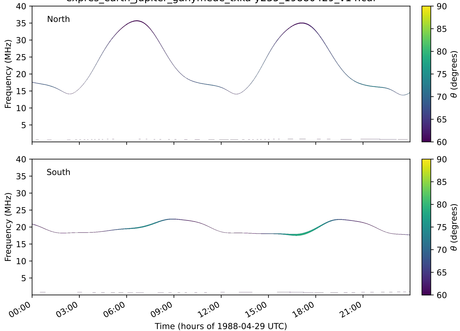
expres_earth_jupiter_ganymede_txka-y235_19880429_v14.cdf
