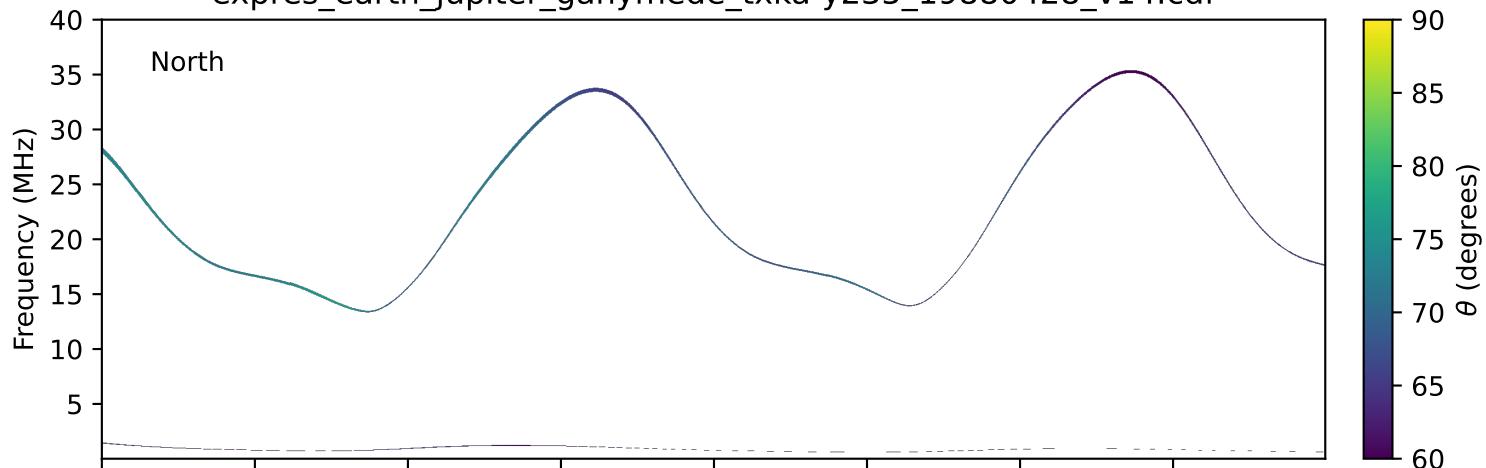
expres_earth_jupiter_ganymede_txka-y235_19880428_v14.cdf
