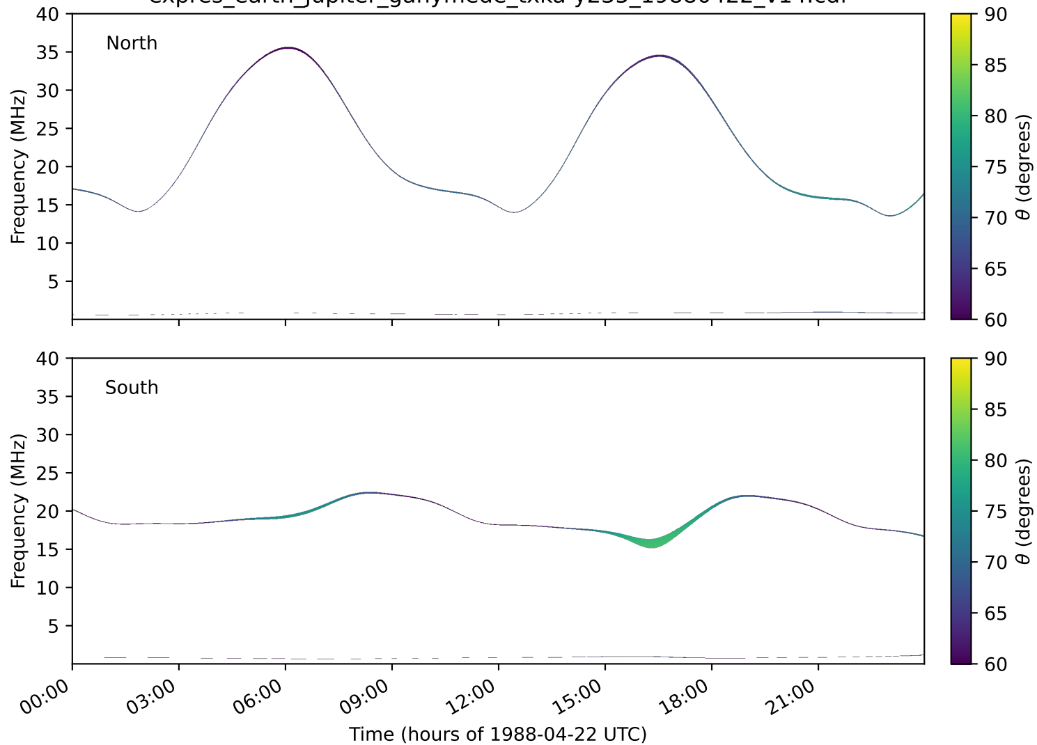
expres_earth_jupiter_ganymede_txka-y235_19880422_v14.cdf
