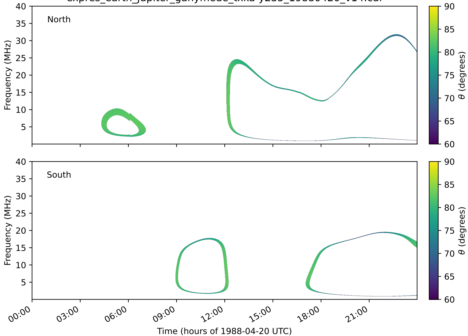
expres_earth_jupiter_ganymede_txka-y235_19880420_v14.cdf
