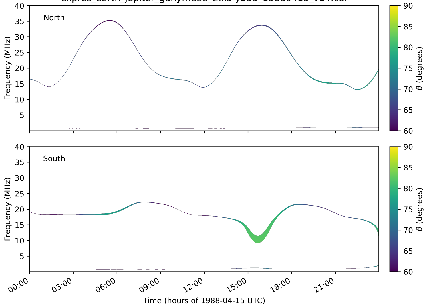
expres_earth_jupiter_ganymede_txka-y235_19880415_v14.cdf
