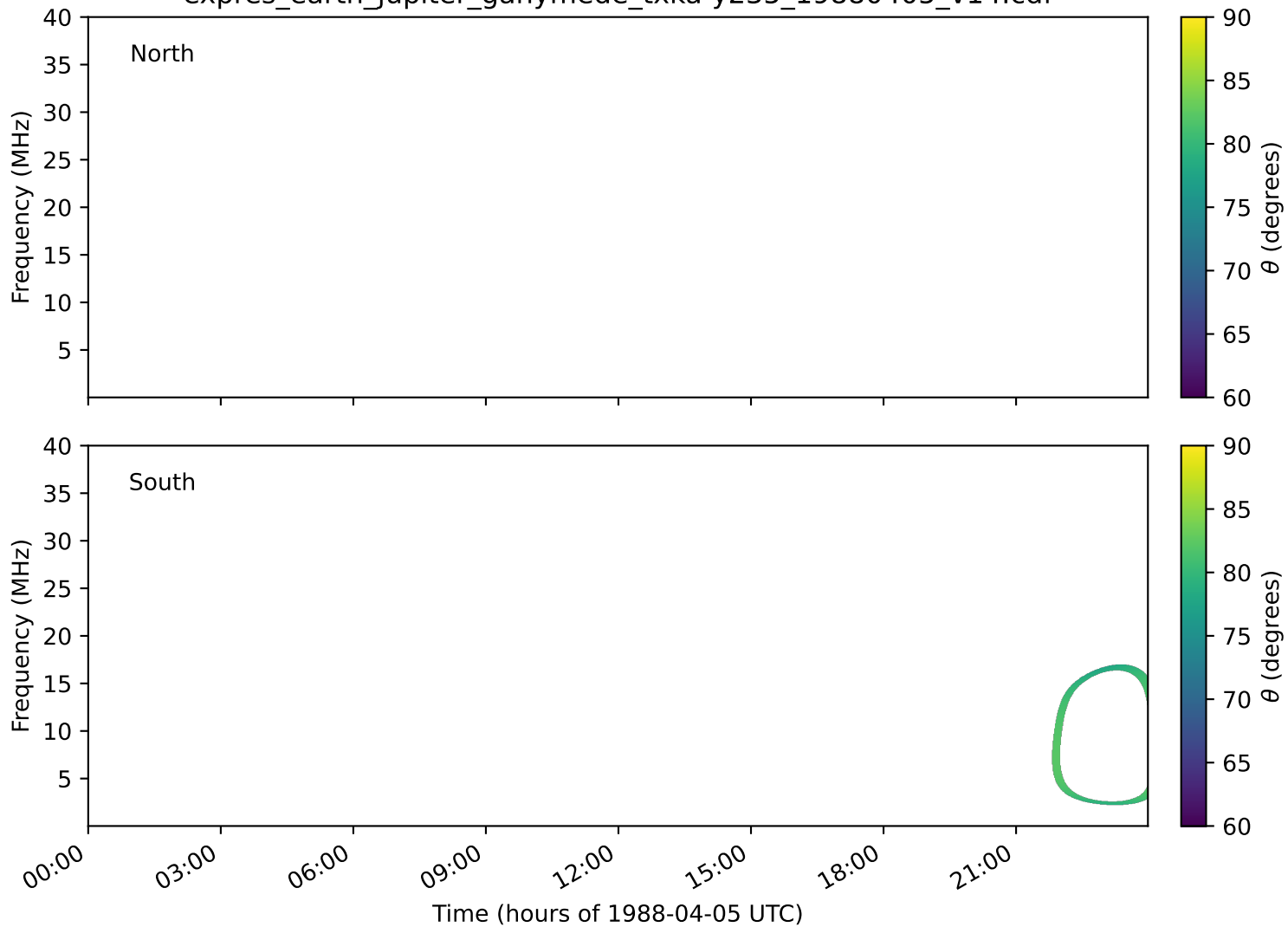
expres_earth_jupiter_ganymede_txka-y235_19880405_v14.cdf
