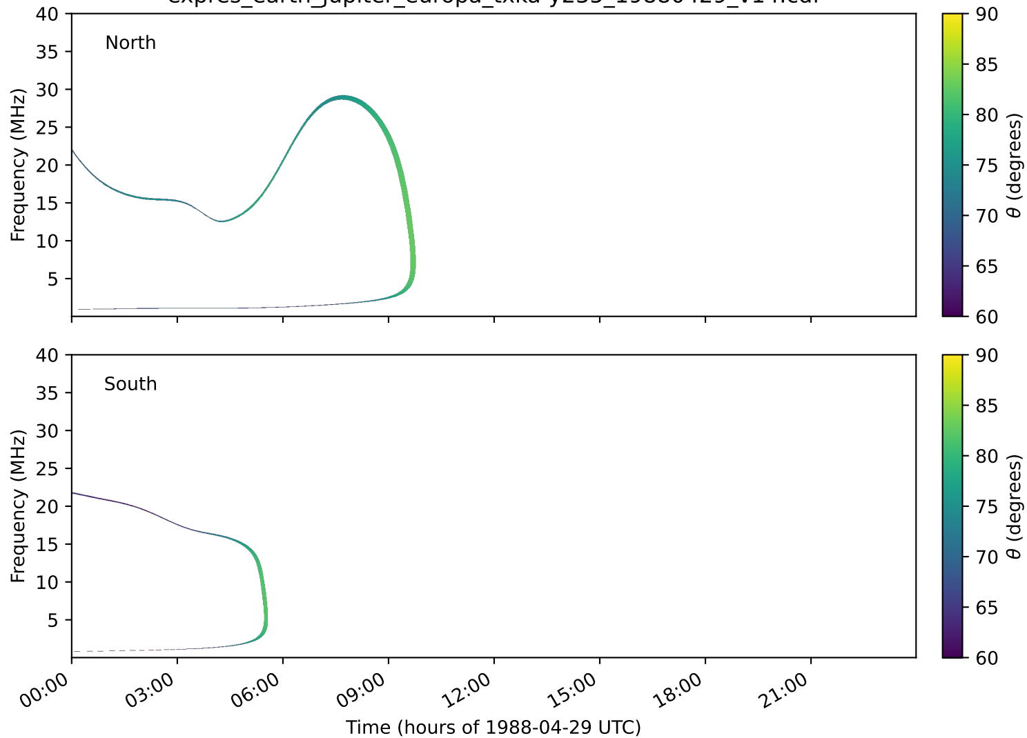
expres_earth_jupiter_europa_txka-y235_19880429_v14.cdf
