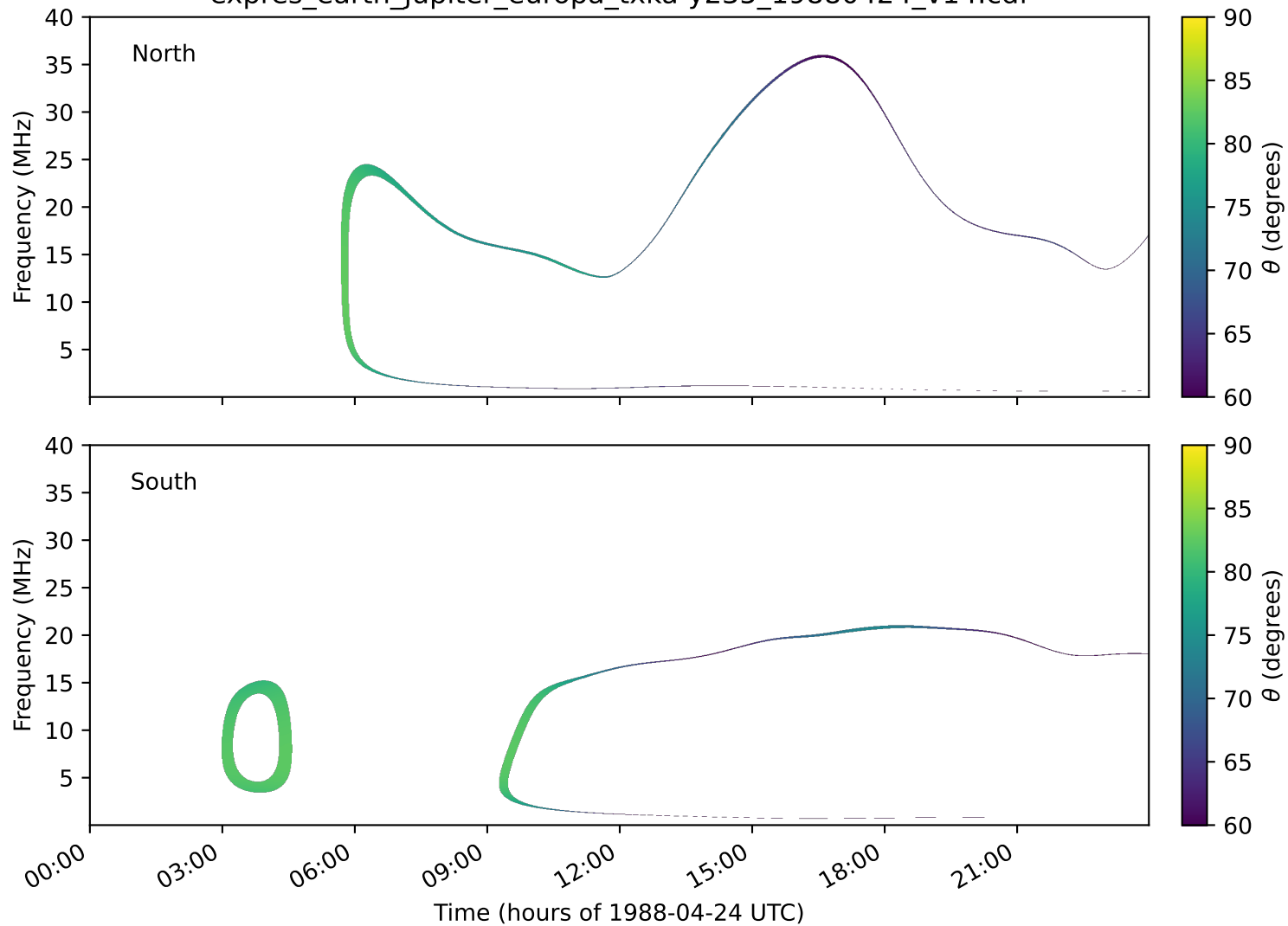
expres_earth_jupiter_europa_txka-y235_19880424_v14.cdf
