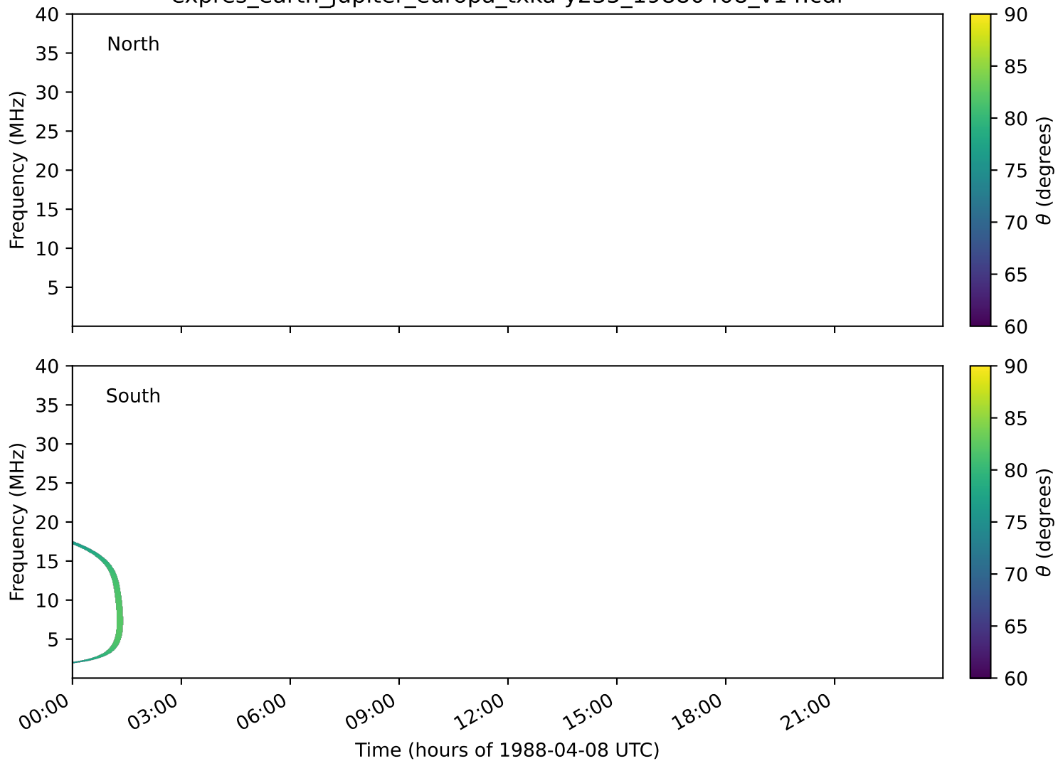
expres_earth_jupiter_europa_txka-y235_19880408_v14.cdf
