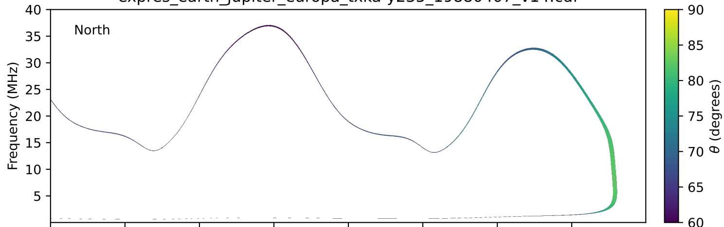
expres_earth_jupiter_europa_txka-y235_19880407_v14.cdf
