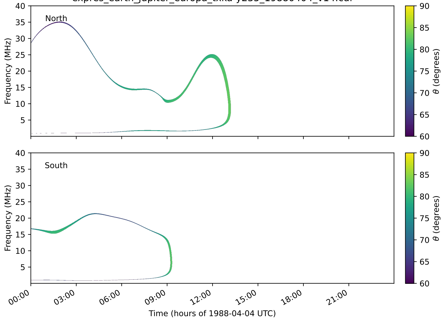
expres_earth_jupiter_europa_txka-y235_19880404_v14.cdf
