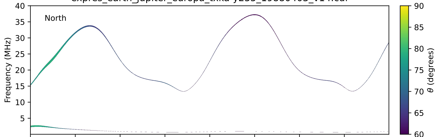
expres_earth_jupiter_europa_txka-y235_19880403_v14.cdf
