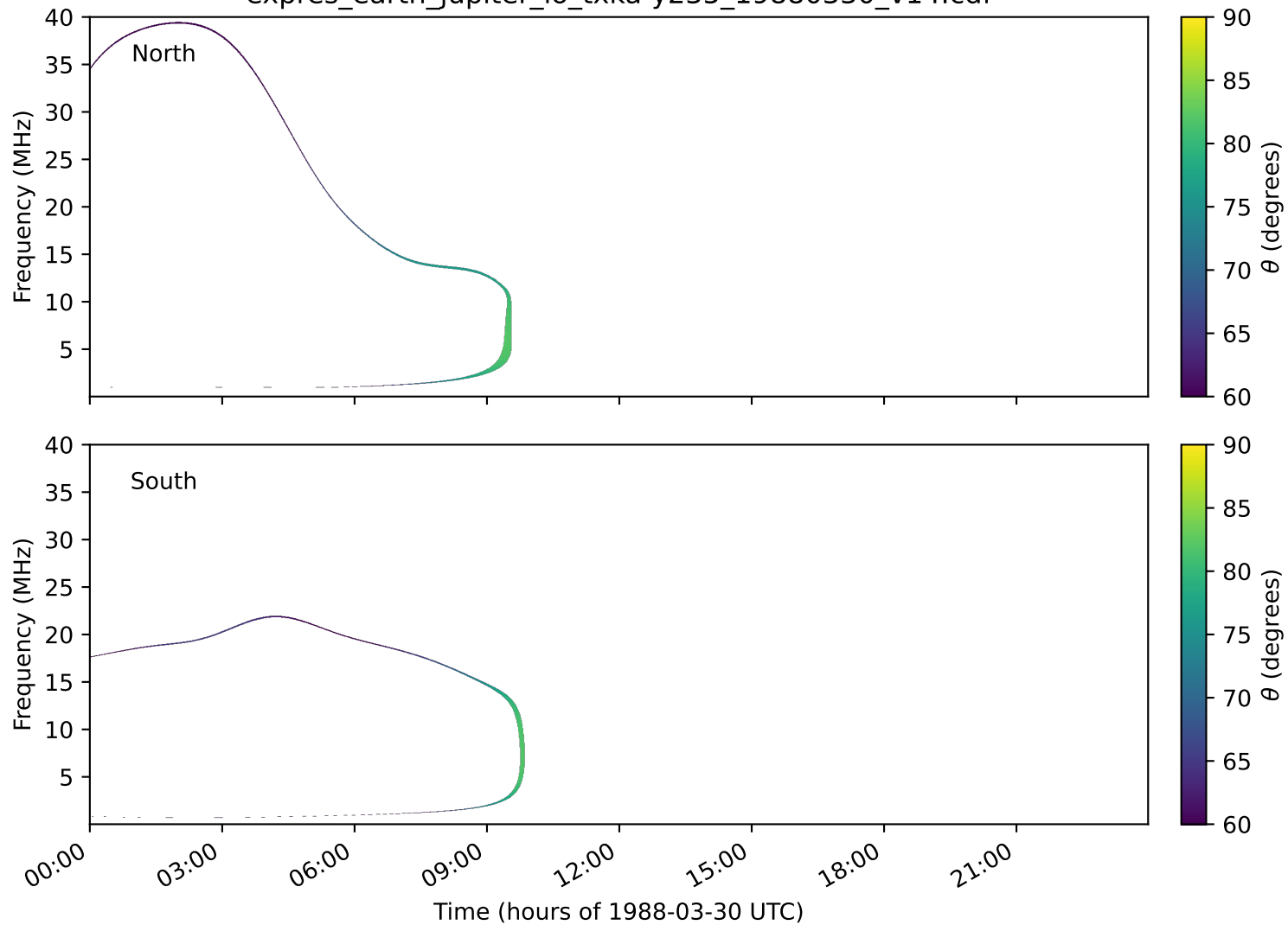
expres_earth_jupiter_io_txka-y235_19880330_v14.cdf
