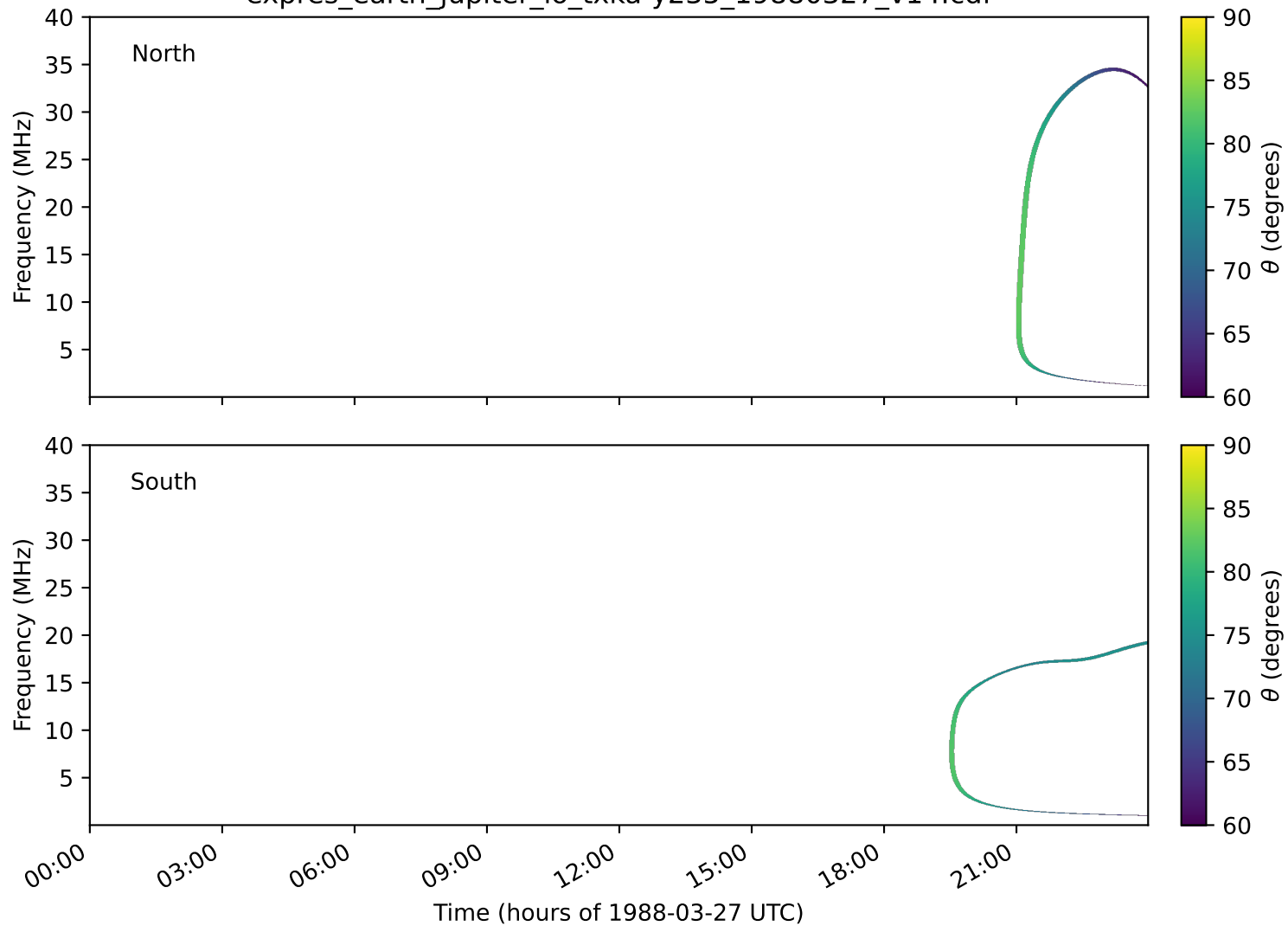
expres_earth_jupiter_io_txka-y235_19880327_v14.cdf
