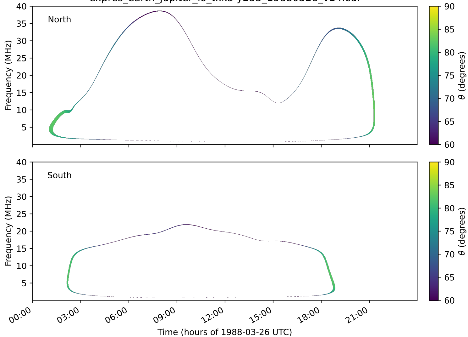
expres_earth_jupiter_io_txka-y235_19880326_v14.cdf
