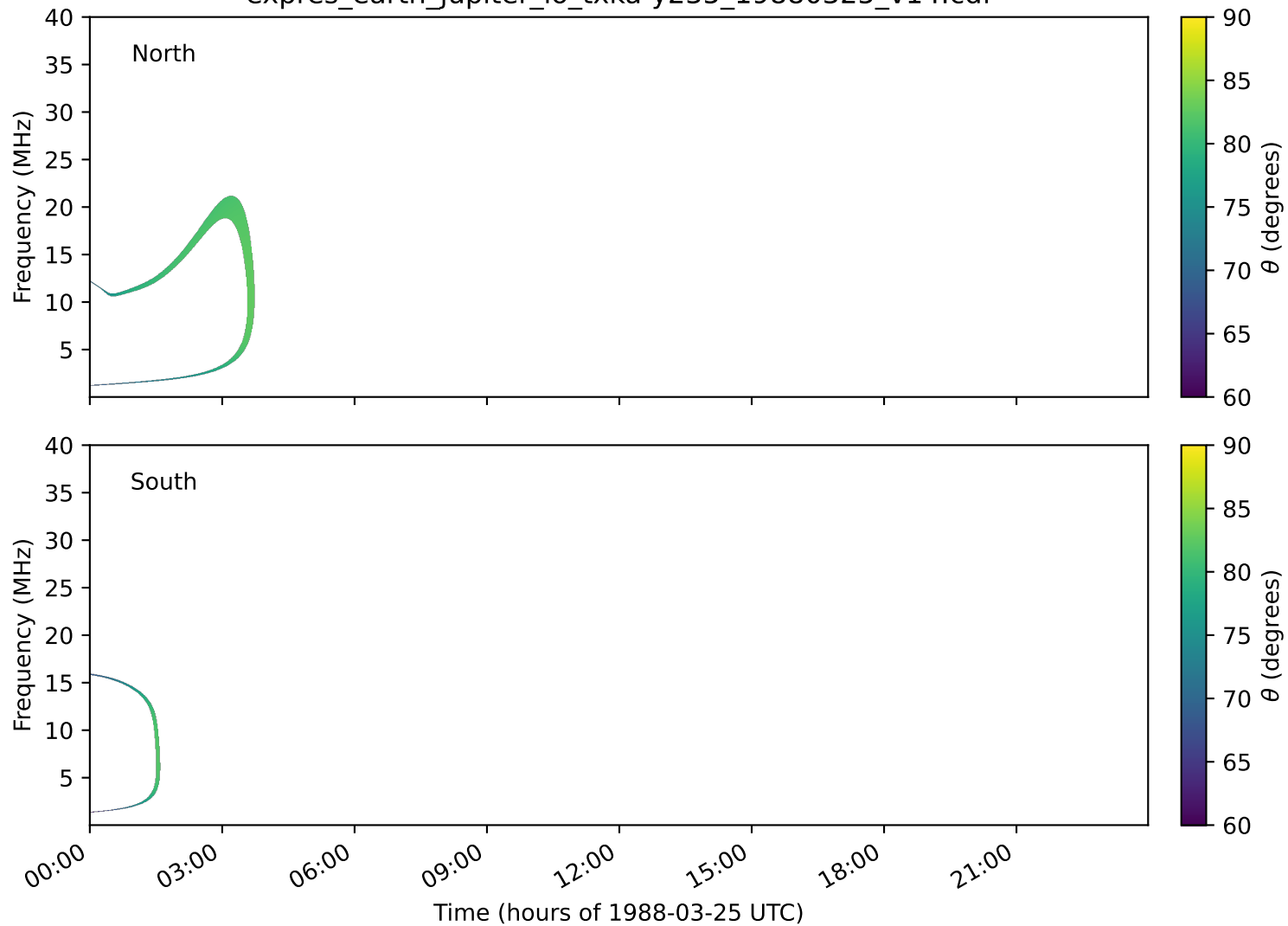
expres_earth_jupiter_io_txka-y235_19880325_v14.cdf
