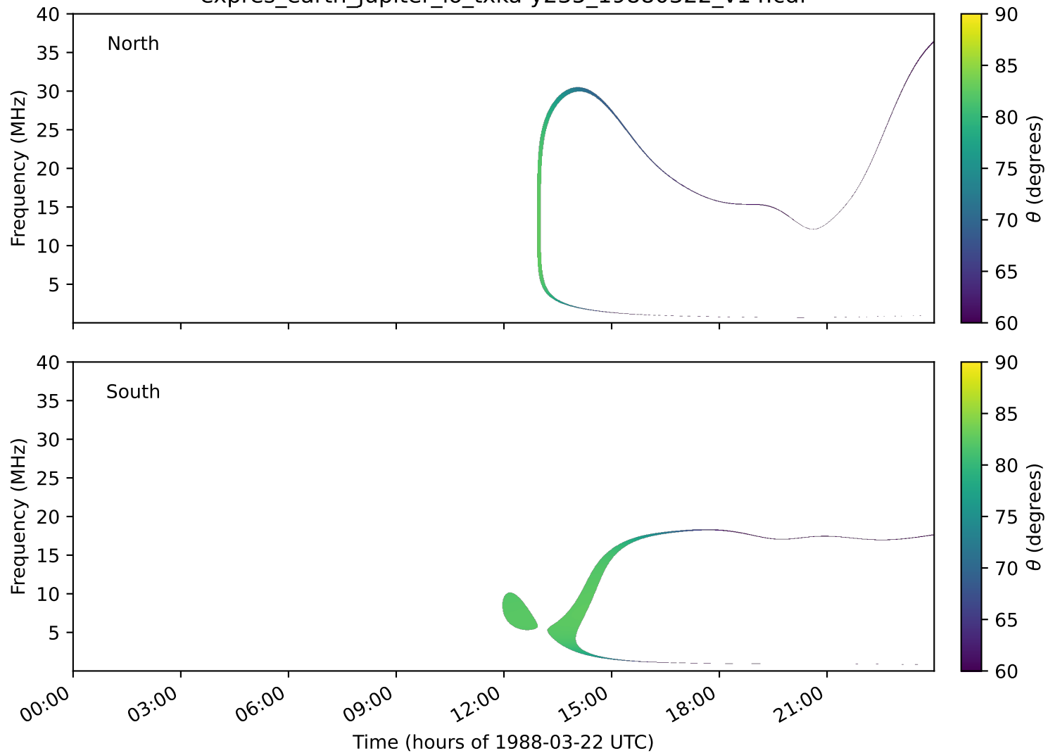
expres_earth_jupiter_io_txka-y235_19880322_v14.cdf
